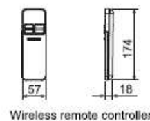
Wireless remote controller
